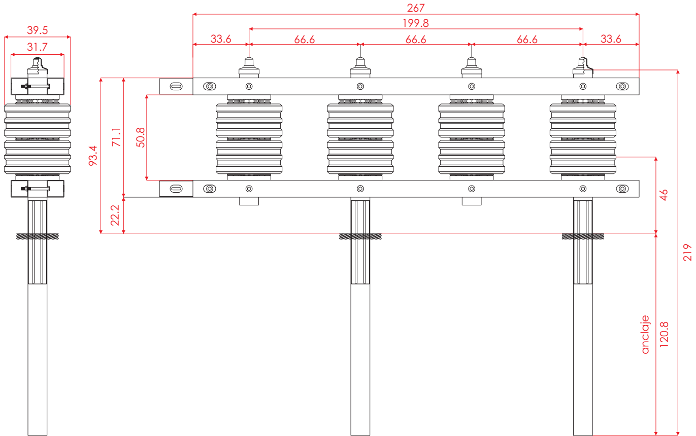
VISTA FRONTAL
