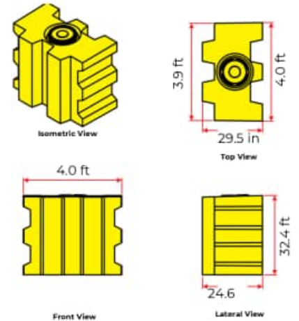
Universal module Capacity 176-gal.
