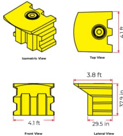
Coupling module Capacity 203-gal.
