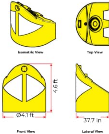
Main module Capacity 248-gal.
